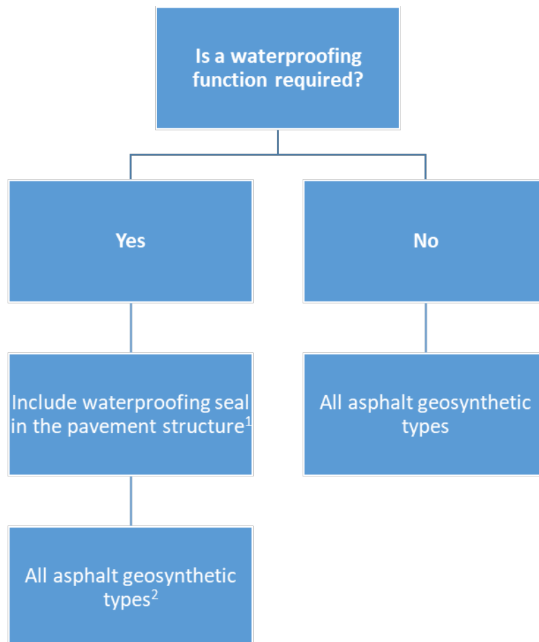
Figure 6.2 – Waterproofing function
