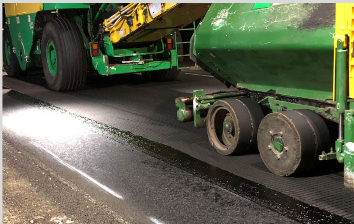
Figure 9.6.3(b) – Example of minimum bitumen pick-up on truck tyres or paving equipment
