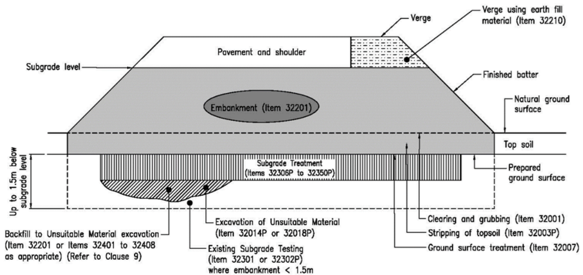
Figure 2.1(c) – Excavation and Embankment to structures
